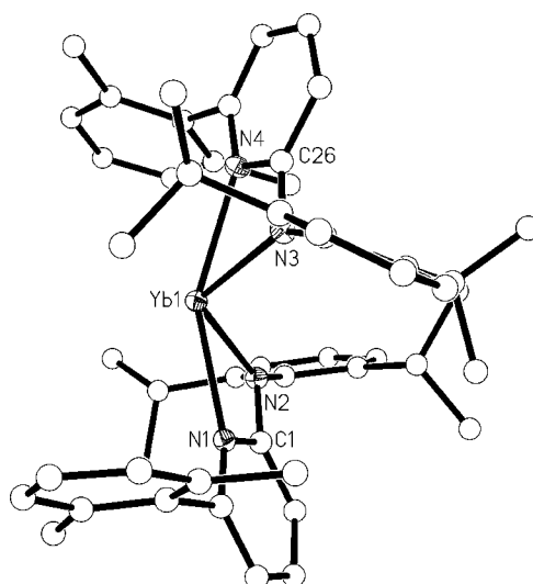
Figure 1. Molecular structure of [\text{Yb}(\text{Ap}')_2] ( 3 ). Hydrogen atoms are omitted for clarity. Selected bond lengths [Å] and angles [°]: N1–Yb1 2.4323(18), N2–Yb1 2.4041(18), N3–Yb1 2.3708(18), N4–Yb1 2.4489(18); N1–Yb1–N2 56.05(6), N1–Yb1–N3 105.89(6), N1–Yb1–N4 151.90(6), N2–Yb1–N3 116.20(6), N2–Yb1–N4 109.36(6), N3–Yb1–N4 56.02(6), C1–Yb1–C26 126.93(6).
