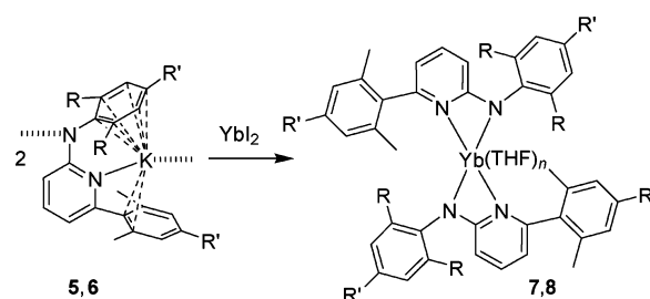
Scheme 4. Synthesis of 7 and 8 ( 5 , 7 : n = 1, R = i Pr; R' = H; 6 , 8 : n = 2, R = R' = Me) by metathesis reactions.
