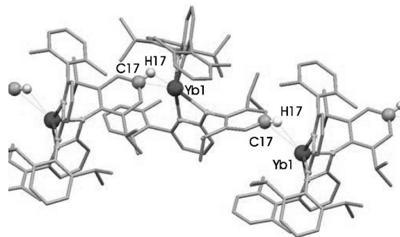
Figure 2. X-ray structure of 3 showing intermolecular agostic interactions [Yb1...C17 2.981(2), Yb1...H17 2.56(3) Å].
